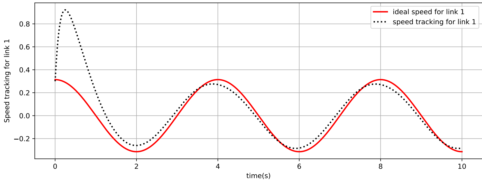
Speed Tracking Performance ( S=1 , S1=1 , m=5 )
